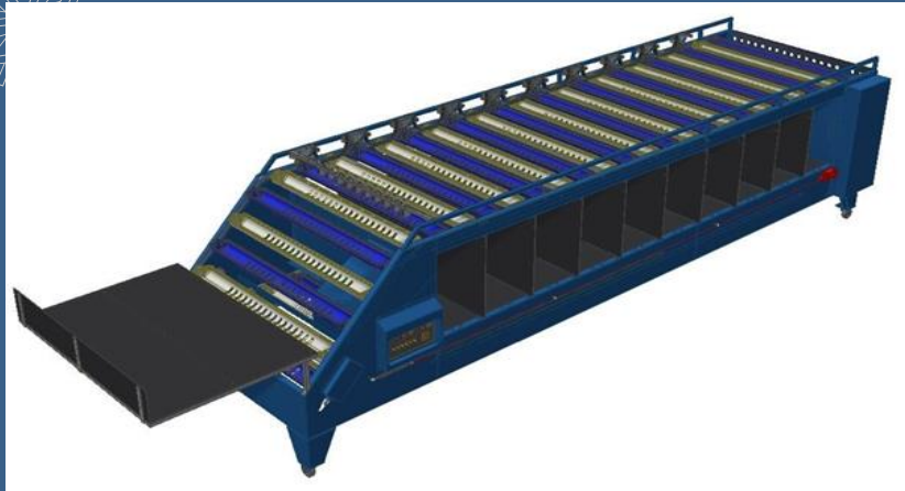
Jamafa dual length grading machine equipped with 1 loading table
